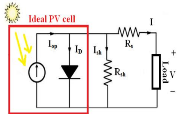
Figure 1: An equivalent circuit of the PV.
