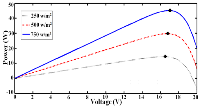
Figure 2: Relationship between output voltage and power of the PV cell under different irradiation conditions.
